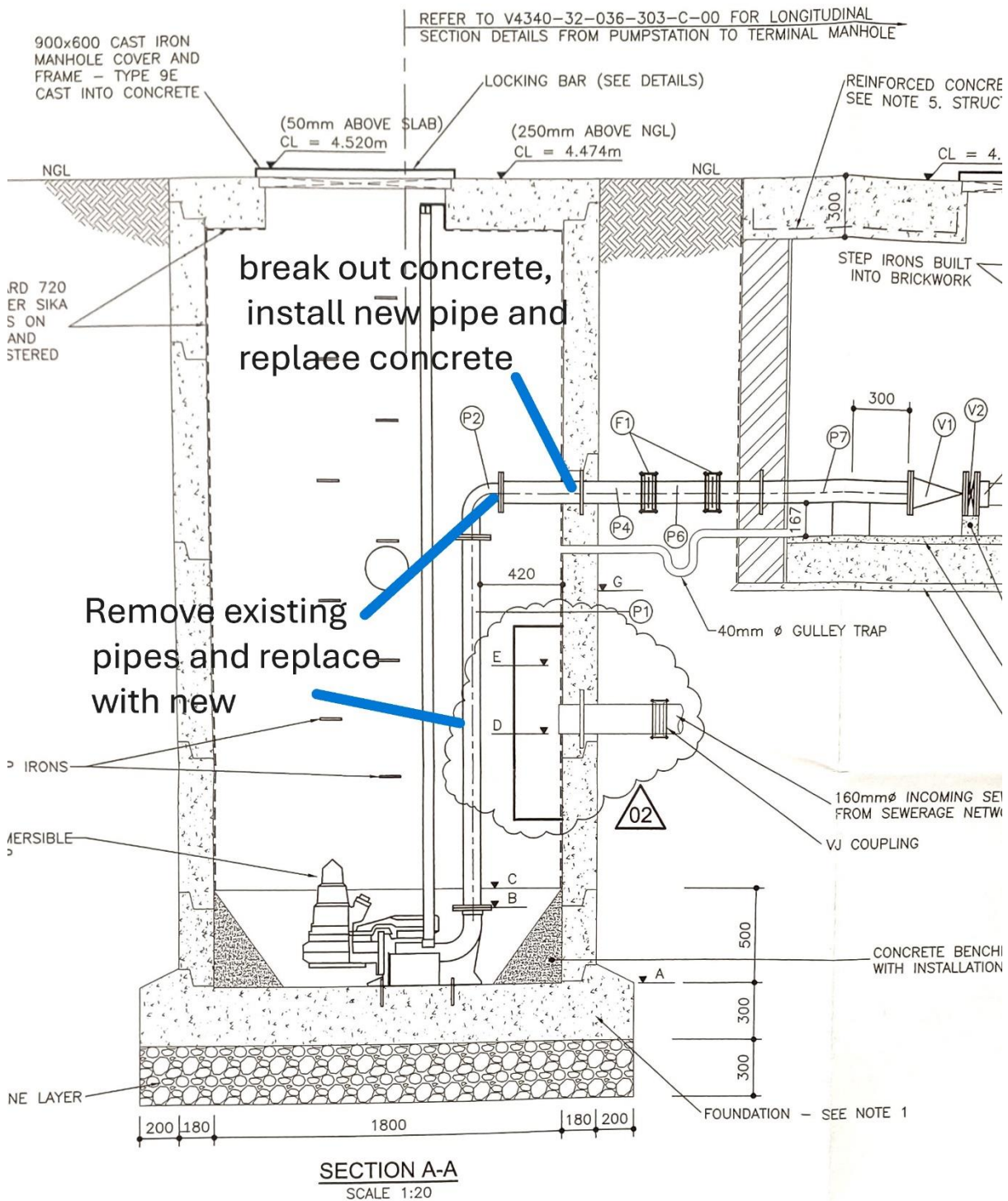
Figure 1 Typical pumpstation detail
