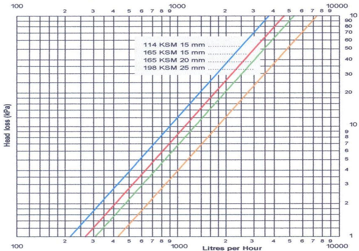
Head loss curves (Typical) 15 & 20mm KSM T water meters
