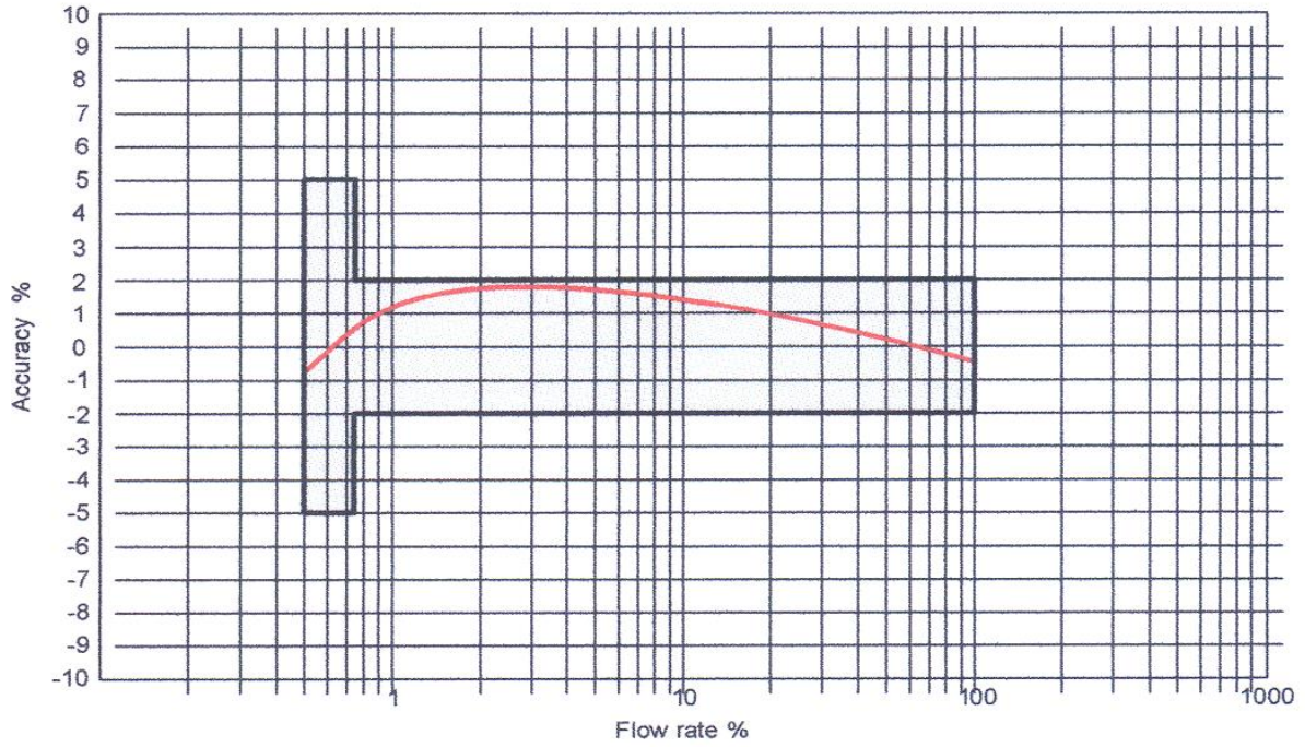
Typical flow graph for volumetric meters
